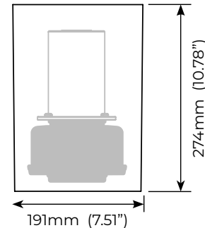
7" Cylinder Reflector shown with VA6 Lamp
